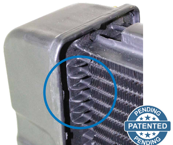
Radiator Image with reinforcement clips
